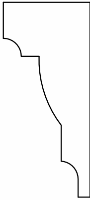
② Wall Band (decoramould 012) 1 1/2" = 1'-0"
