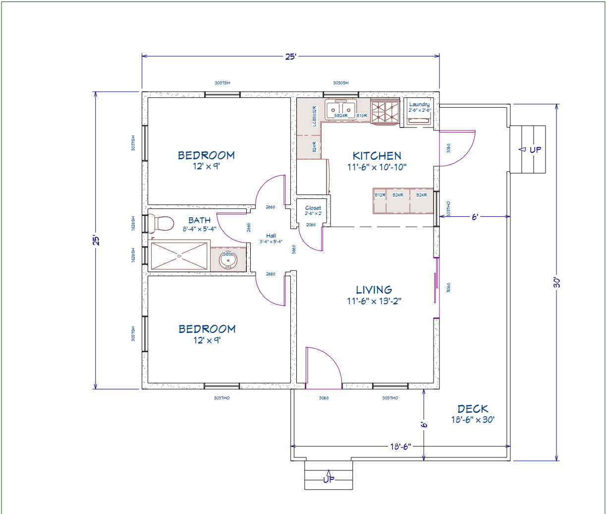
LIVING AREA 625 sq ft
